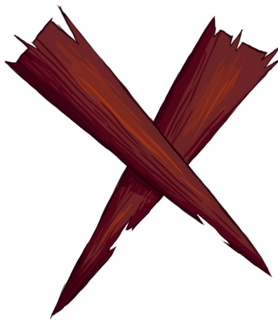
Orlek's Symbol
