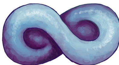
Ewen's Symbol
